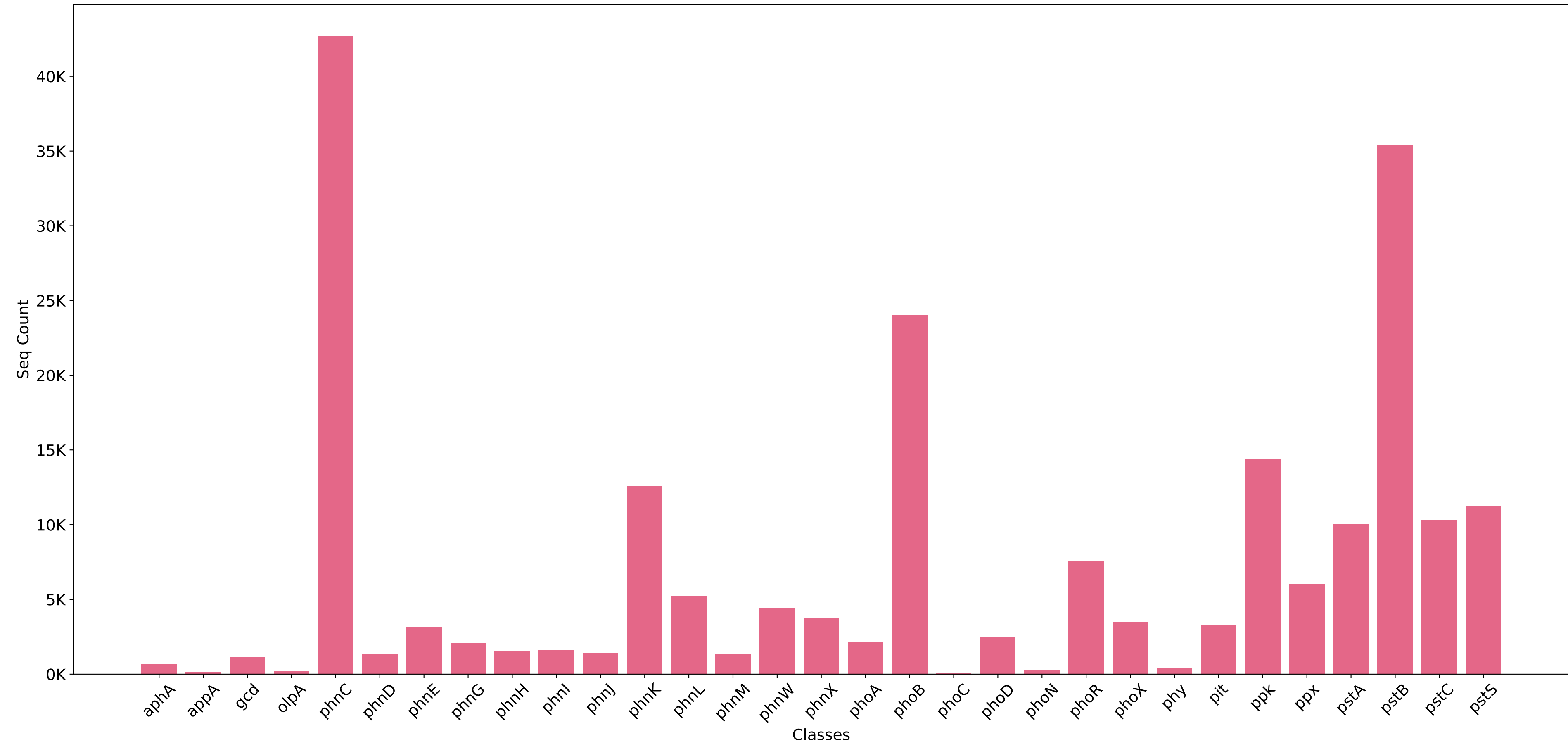
31 Classes (Positives)
